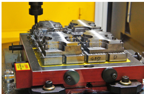
Gang part setups together and still machine 5 sides
